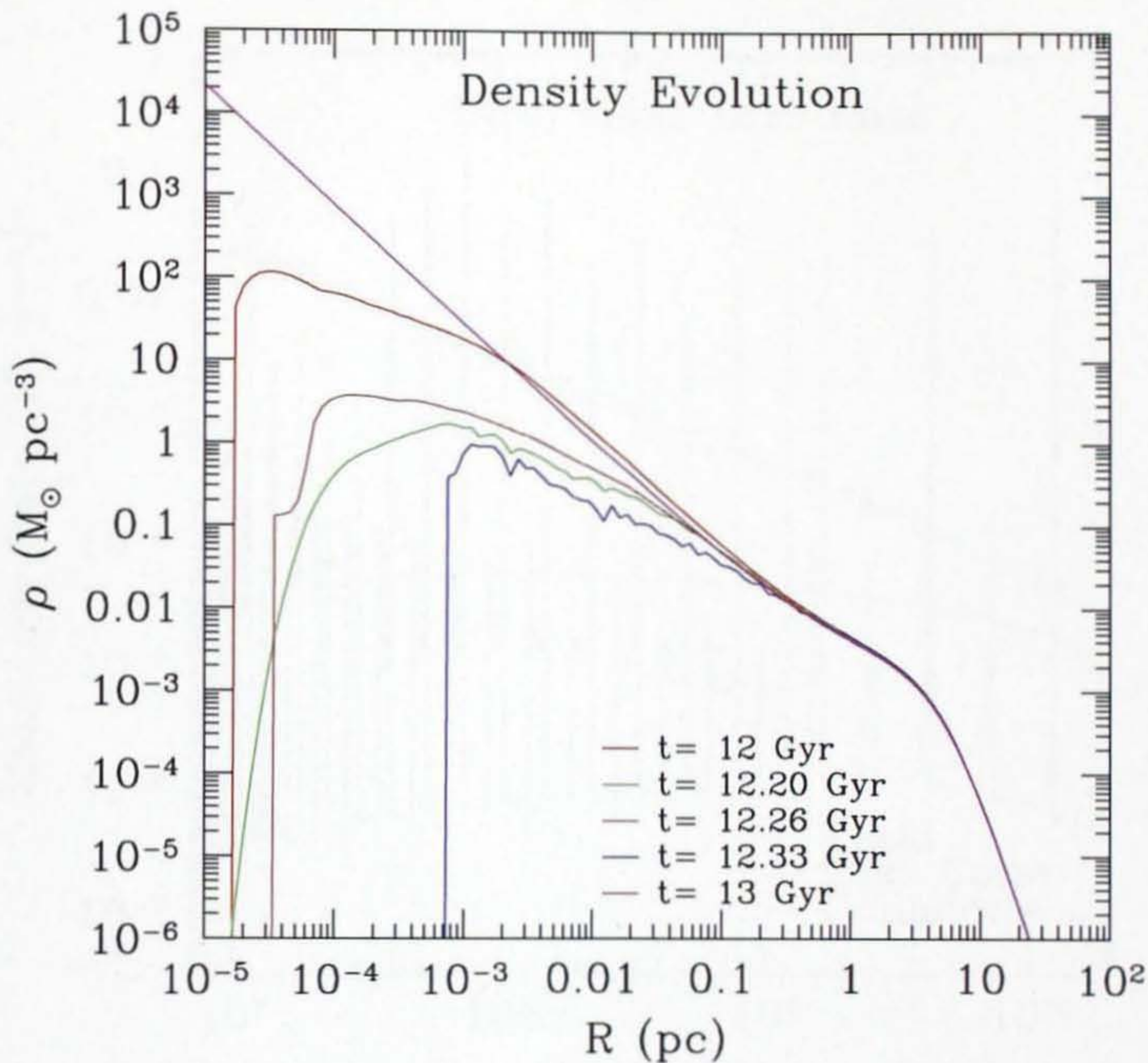
Fig. 3.— The density profile of the mass group at each of the star's evolutionary phases. Red is the main sequence phase, green is immediately following the red giant phase, peach is during the horizontal branch phase, blue is the climax of the AGB phase, and magenta is the white dwarf phase. As the stars in the mass group evolve, the density changes due to stellar collisions, tidal disruptions, and drift cause by stellar interactions. Tidal disruptions prevent stars from existing within the Roche limit from the center, causing the sudden drop in the density profile. Drift can allow stars to refill these areas when the Roche limit decreases, as with the horizontal branch and white dwarf stars. Evidence of this is also seen in the red giant profile due the stellar radius having just passed its peak.
