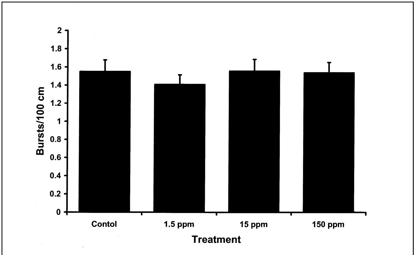
Figure 5. Effect of acute (24 hour) exposure to 2,4-D on the number of swimming bursts required for southern leopard frog tadpoles to cover the 100 cm swimming track. Bars a treatment means and error bars are equal to one standard error.
