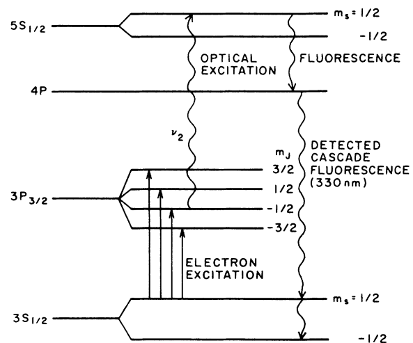
FIG. 1. Na atoms are excited from 3S_{1/2}(m_S' = \frac{1}{2}) to the Zeeman-split m_J levels of the 3P_{3/2} state, and the relative populations in these levels are probed by tuning a laser to excite from 3P_{3/2} to 5S_{1/2} and observing the resultant 4P cascade fluorescence.
