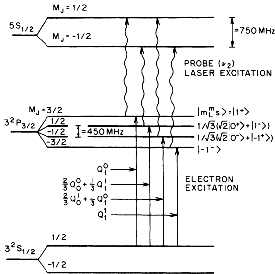
FIG. 4. Energy levels and states of Na involved in this experiment. The 3P_{3/2}(m_J) levels are decomposed into their m_S and m_L components, and the Q_{|\Delta m_L|}^{|\Delta m_S|} cross section relevant for excitation to each m_J is indicated.
