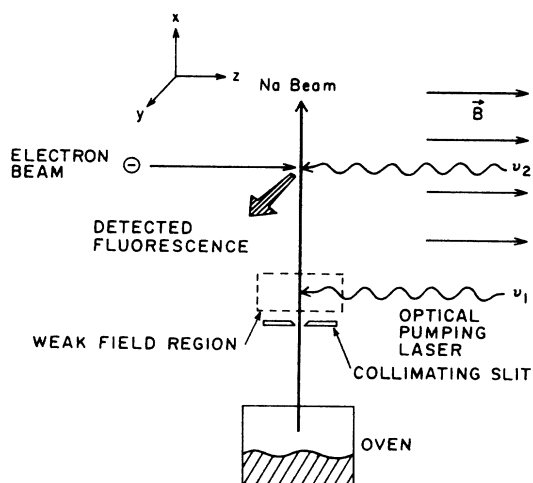
FIG. 3. Sketch of the basic experimental setup. The optical pumping of the sodium beam occurs in a \sim 5 G field, while the electron-atom collisions occur in a field of B \approx 220 G.
