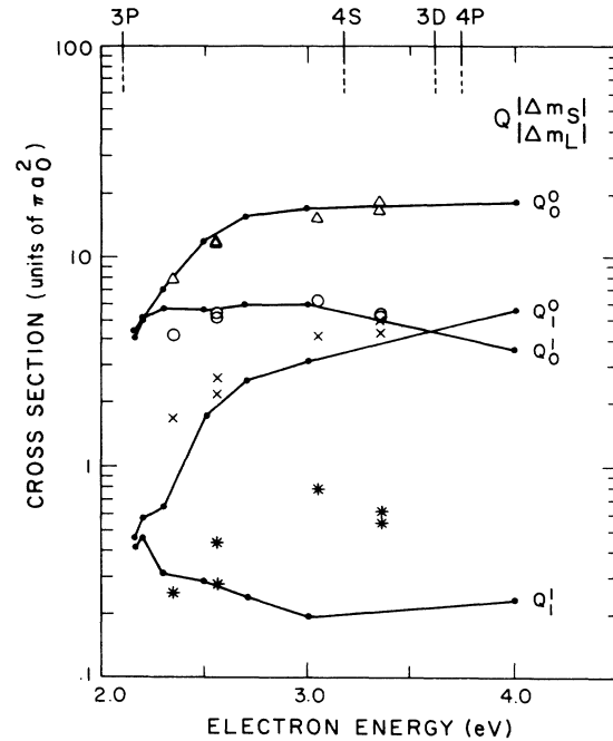
FIG. 5. Partial cross sections Q_{|\Delta m_L|}^{|\Delta m_S|} obtained from this work (symbols), compared with the calculated values of Moores and Norcross (solid dots connected by line segments).
