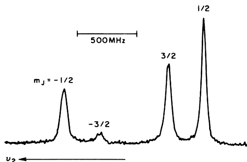
FIG. 2. Detected cascade fluorescence as a function of \nu_2 laser tuning through the 3P_{3/2} - 5S_{1/2} transitions for a mean electron energy of 3.35 eV. Each of the four peaks is labelled by the m_J value of the 3P_{3/2} state being probed (see Fig. 5). The data points are separated by 4 MHz, and the integration time per point is 6 s.
